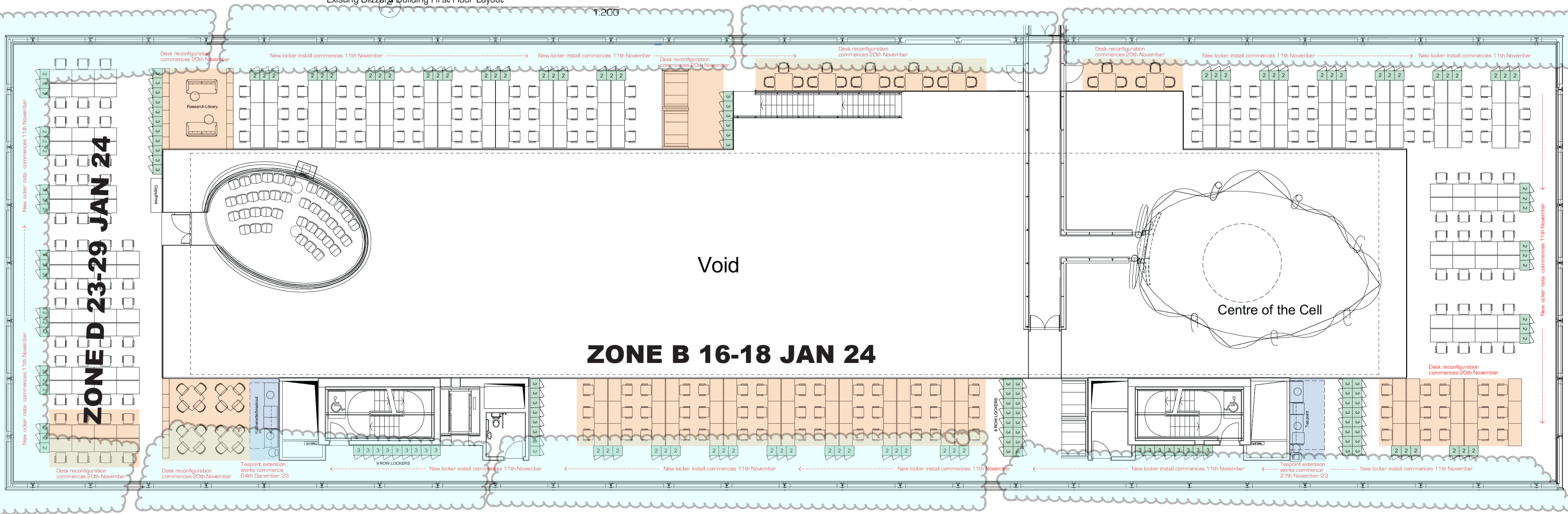
3 Proposed Blizzard First Floor Layout 1:100
