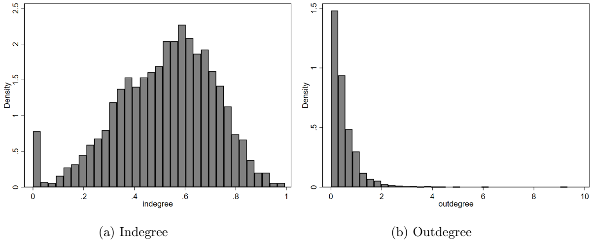
Figure 1: Degree Distributions
