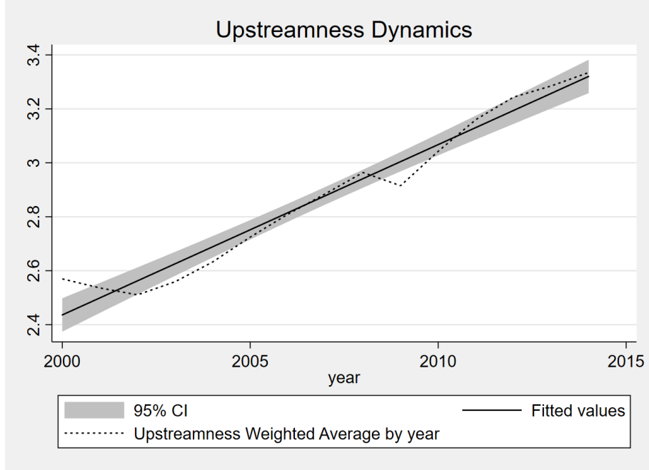
Figure 8: Upstreamness Dynamics
