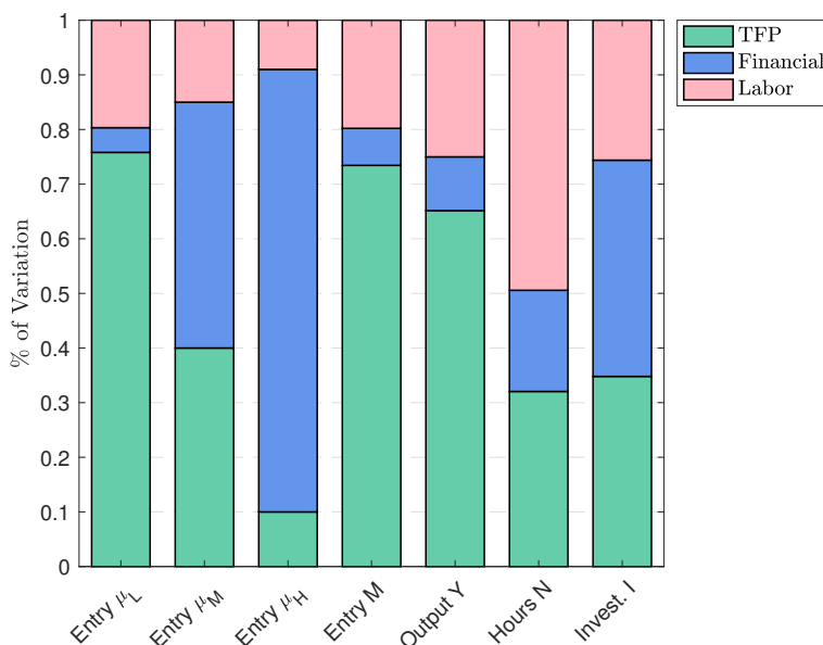
FIGURE 12: VARIANCE DECOMPOSITION
