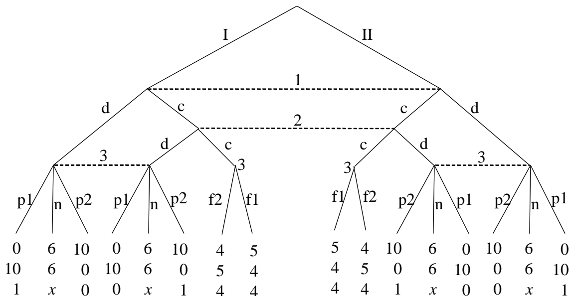
FIGURE 1. A PEACE NEGOTIATION GAME THE VECTORS GIVE UTILITY PAYOFFS FOR PLAYERS 1, 2 AND 3, IN THAT ORDER, FOR EACH PATH.
